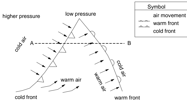
Figure 2.3. Storm as it appears on weather map in the northern hemisphere
