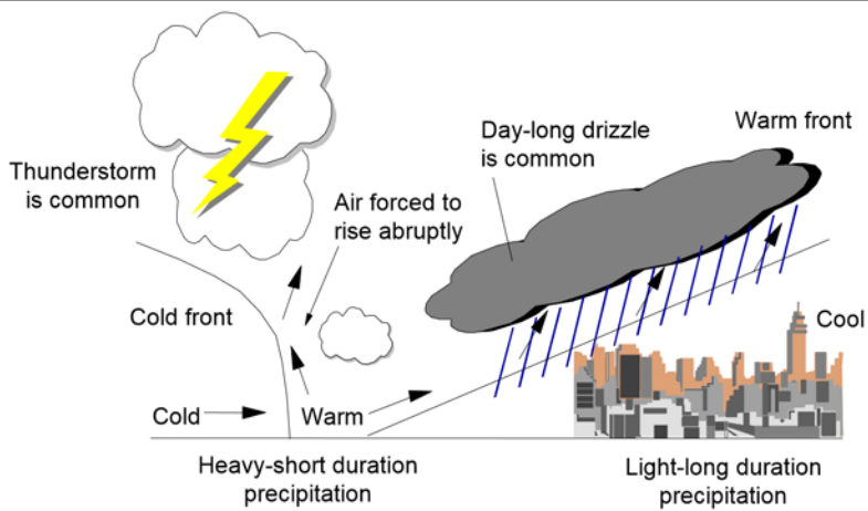
Figure 2.4. Cyclonic storms in mid-latitude; cross-section from A to B of Figure 2.3
